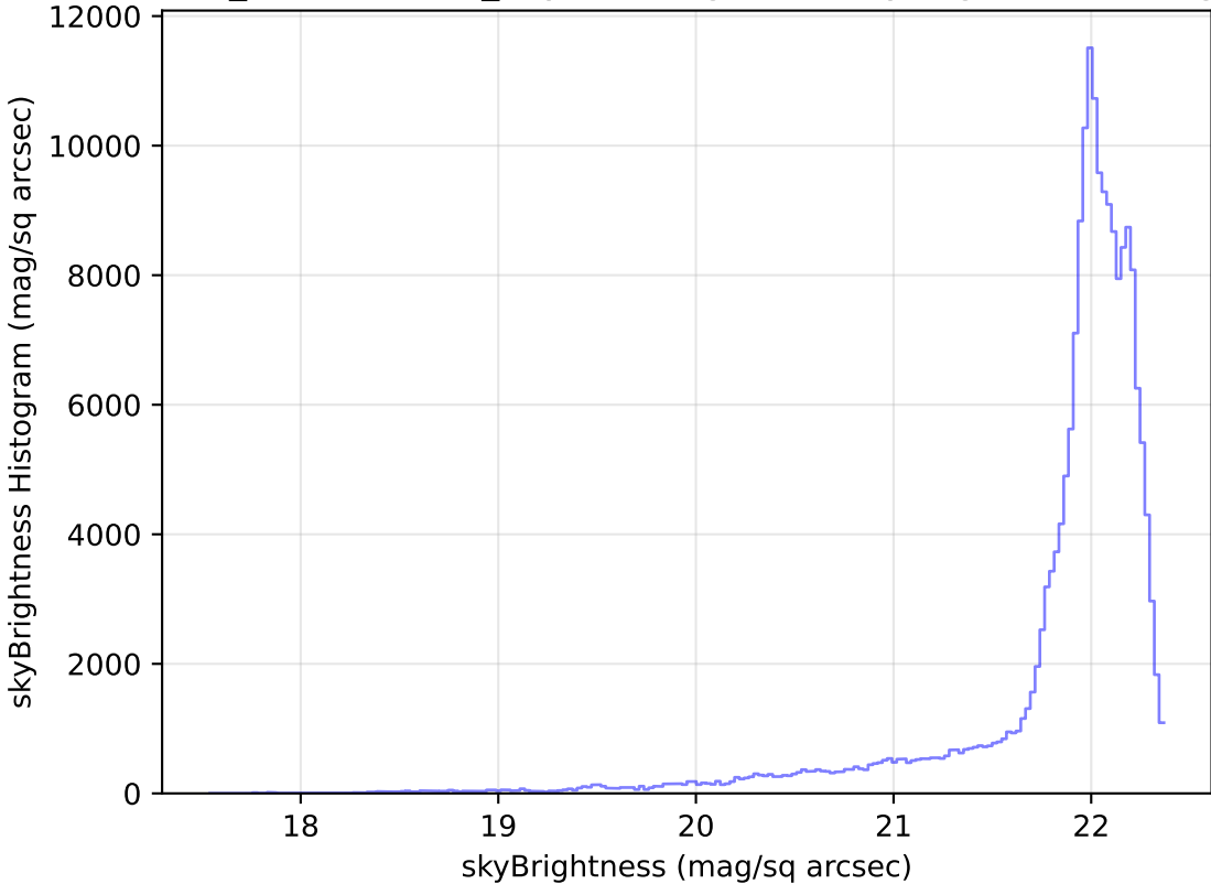
weather_cloudso8v3.4_10yrs WFD g band: skyBrightness Histogram
