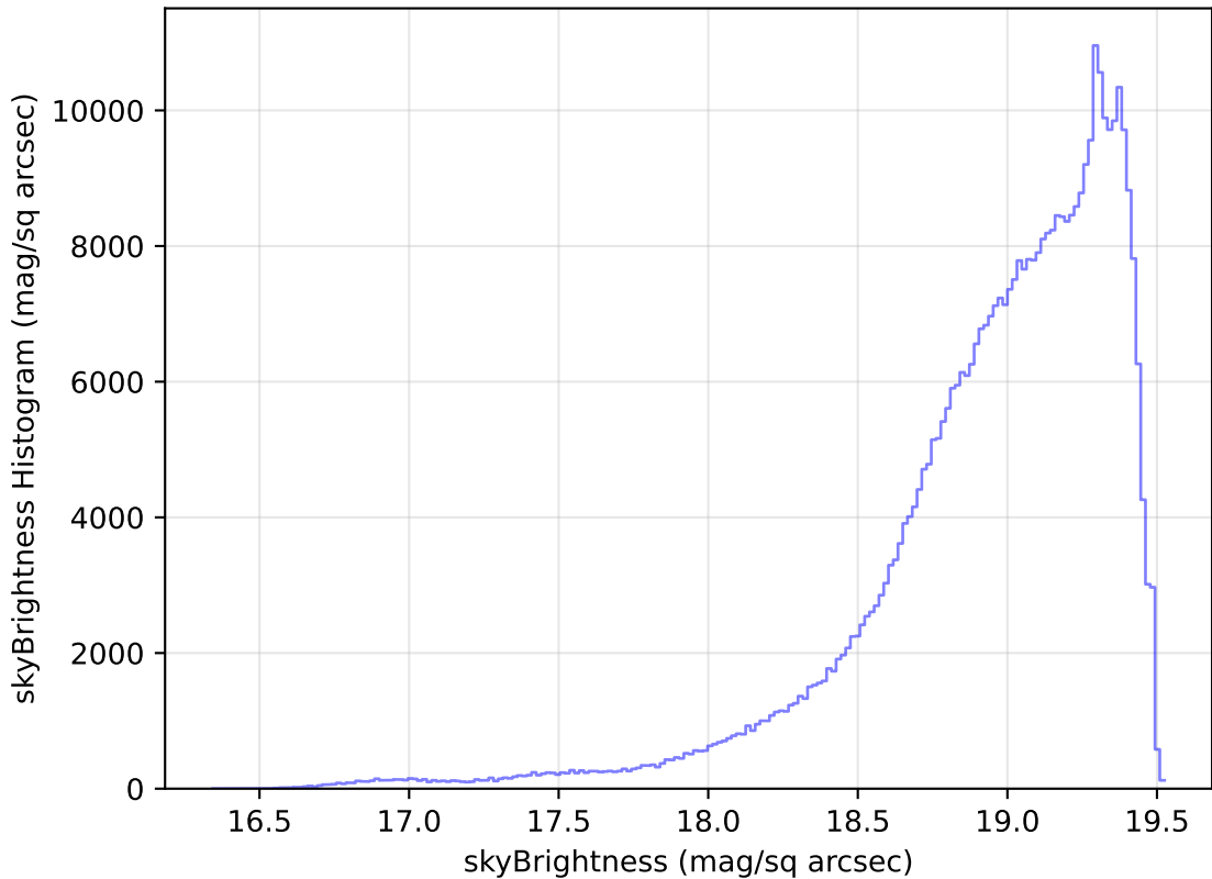
weather_cloudso8v3.4_10yrs All sky z band: skyBrightness Histogram
