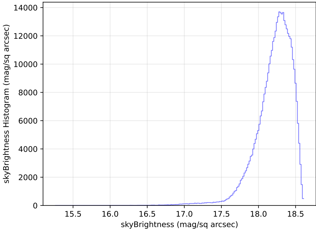
weather_cloudso8v3.4_10yrs All sky y band: skyBrightness Histogram
