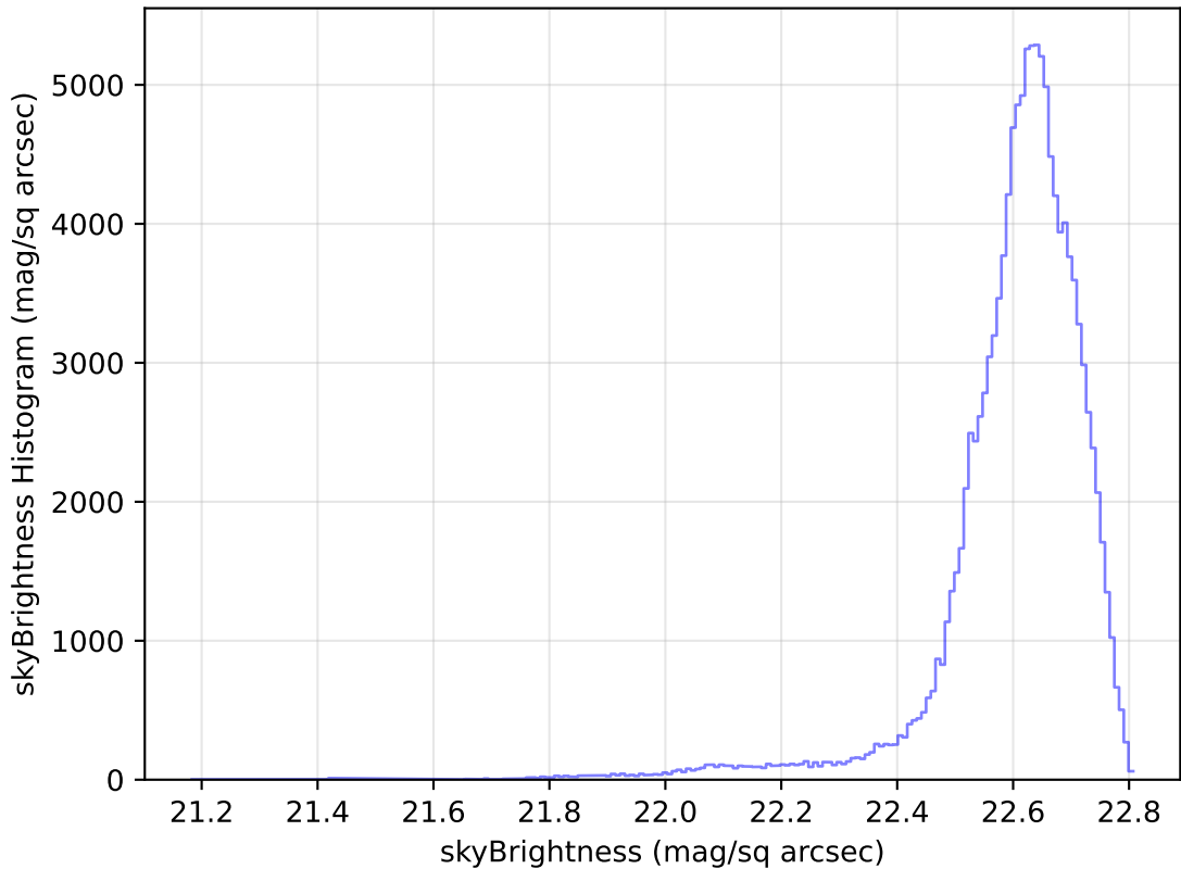
weather_cloudso8v3.4_10yrs All sky u band: skyBrightness Histogram
