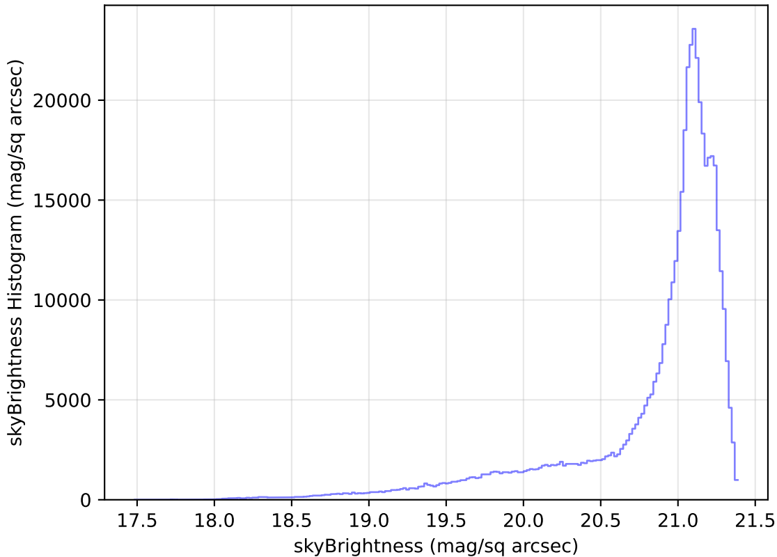
weather_cloudso8v3.4_10yrs All sky r band: skyBrightness Histogram
