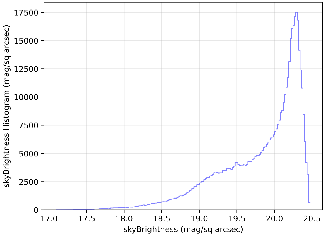
weather_cloudso8v3.4_10yrs All sky i band: skyBrightness Histogram
