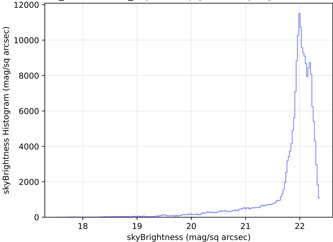
weather_cloudso8v3.4_10yrs All sky g band: skyBrightness Histogram
