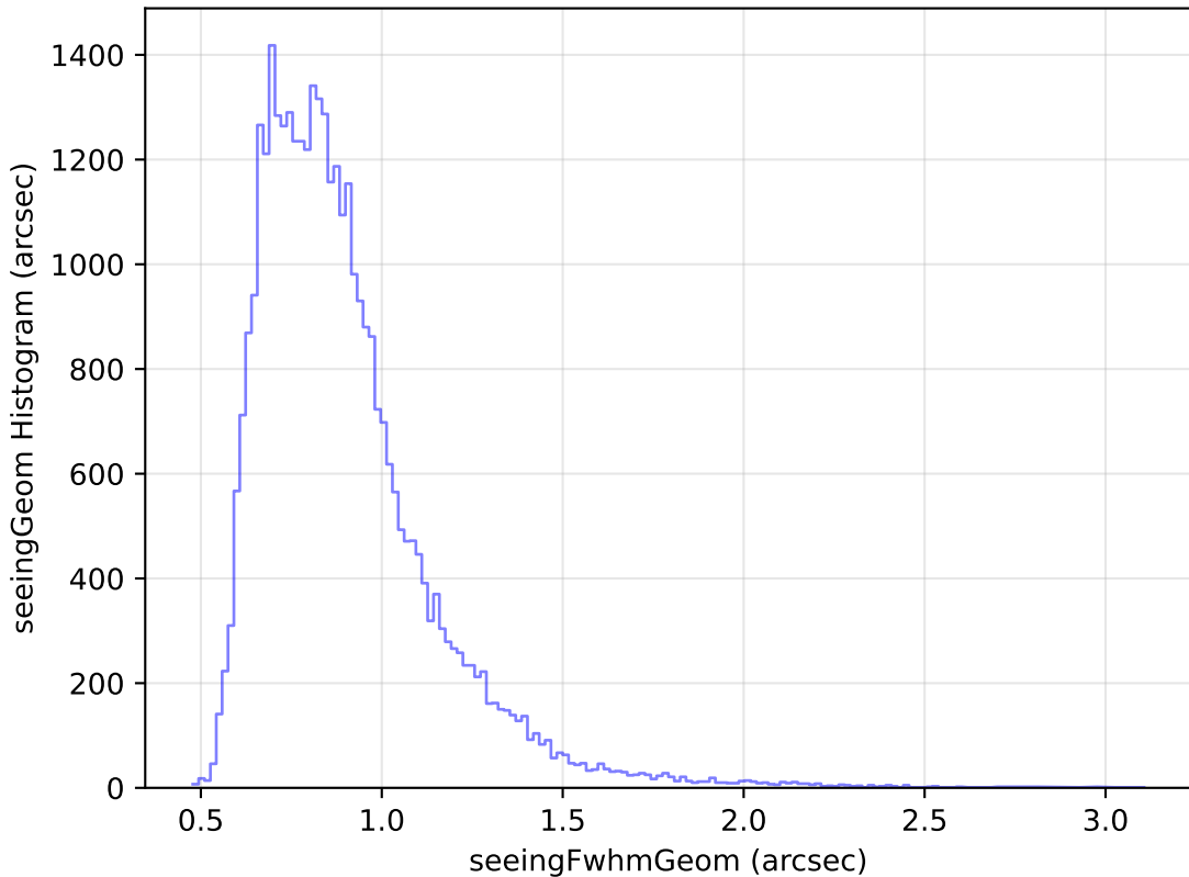
weather_cloudso8v3.4_10yrs Yr 1 z band: seeingGeom Histogram
