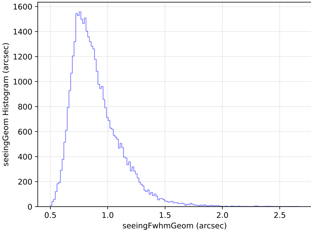
weather_cloudso8v3.4_10yrs Yr 1 y band: seeingGeom Histogram
