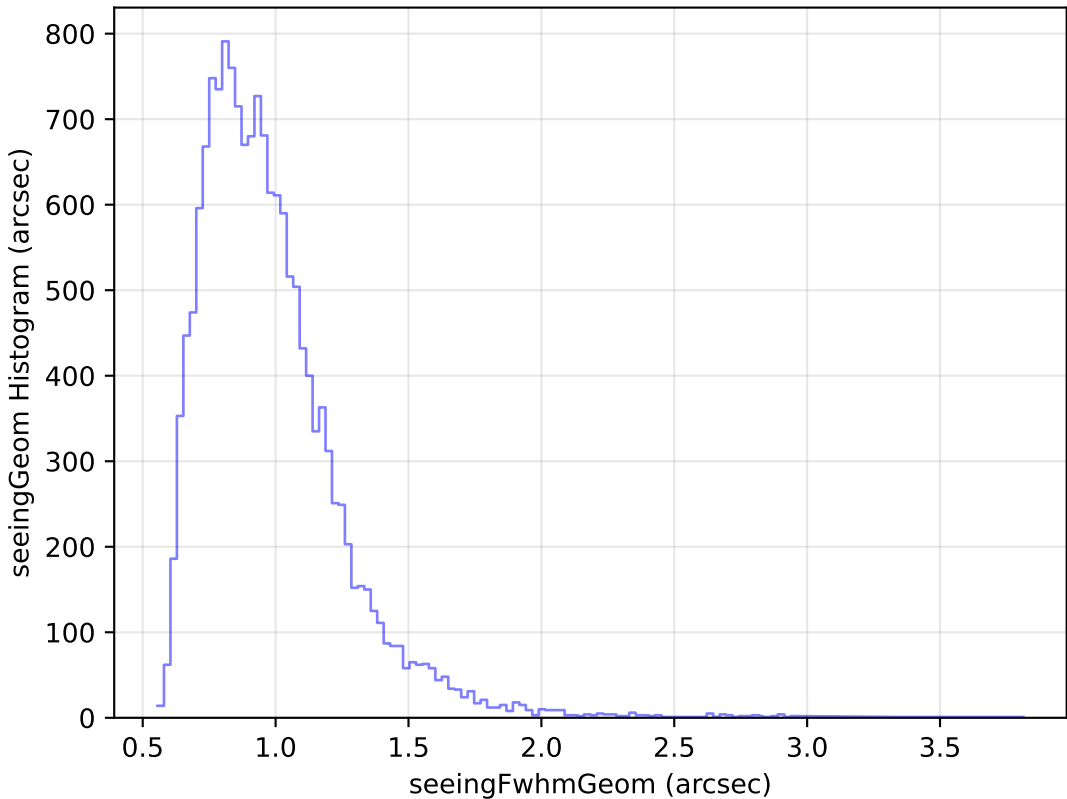
weather_cloudso8v3.4_10yrs Yr 1 u band: seeingGeom Histogram
