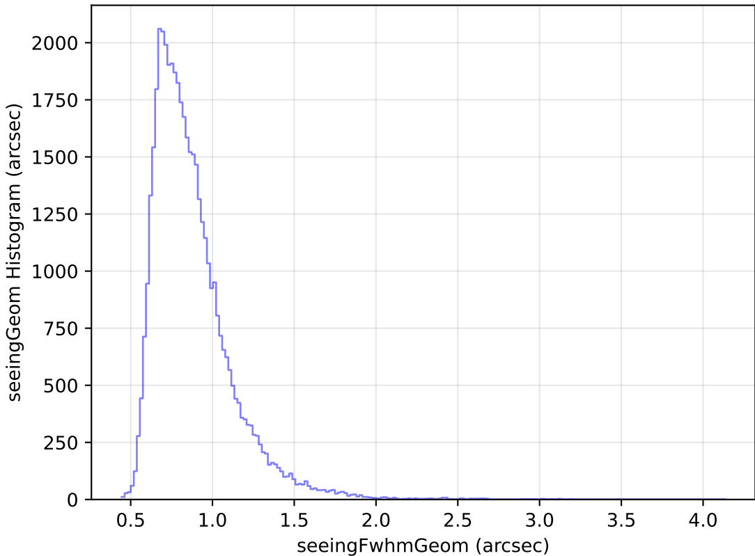
weather_cloudso8v3.4_10yrs Yr 1 i band: seeingGeom Histogram
