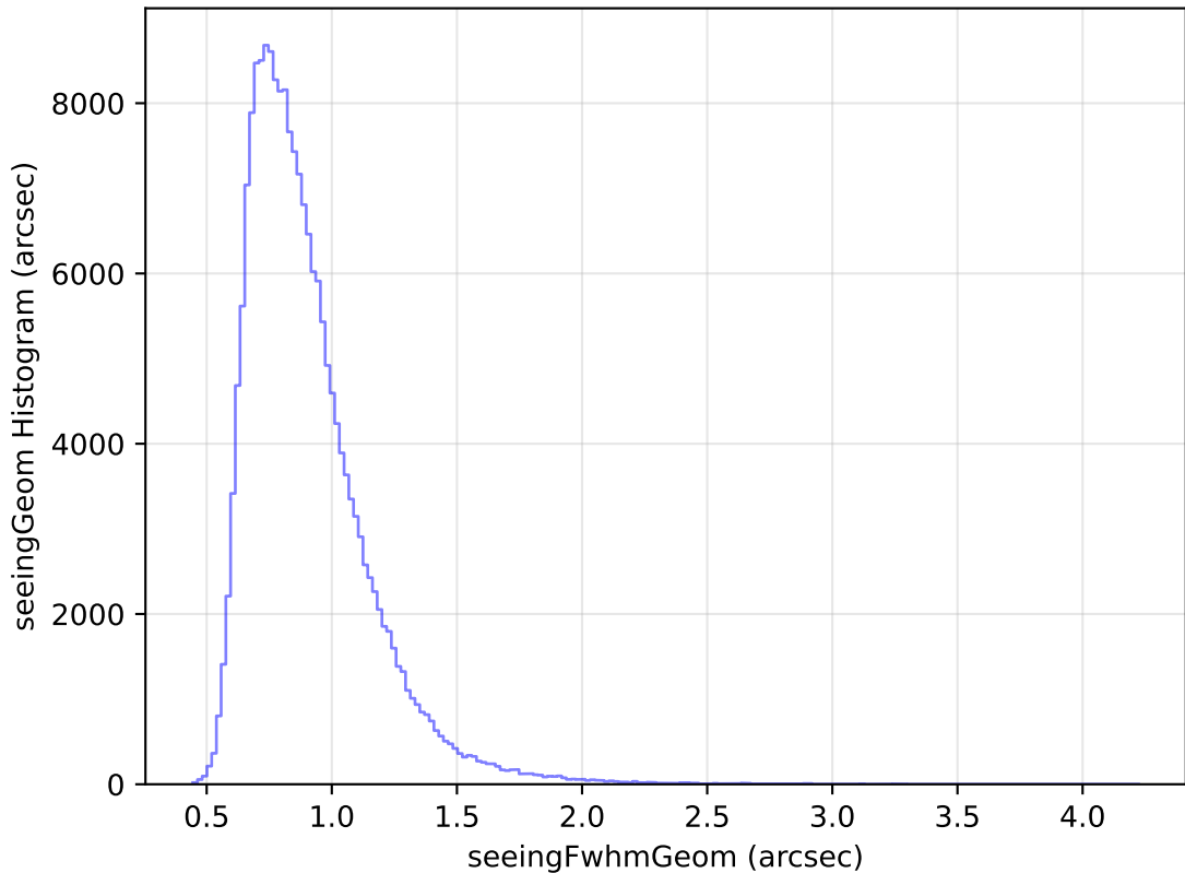
weather_cloudso8v3.4_10yrs Yr 1 all bands: seeingGeom Histogram
