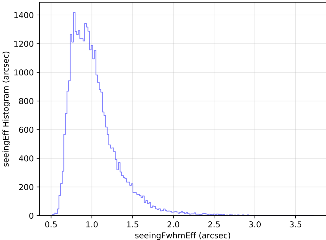
weather_cloudso8v3.4_10yrs Yr 1 z band: seeingEff Histogram
