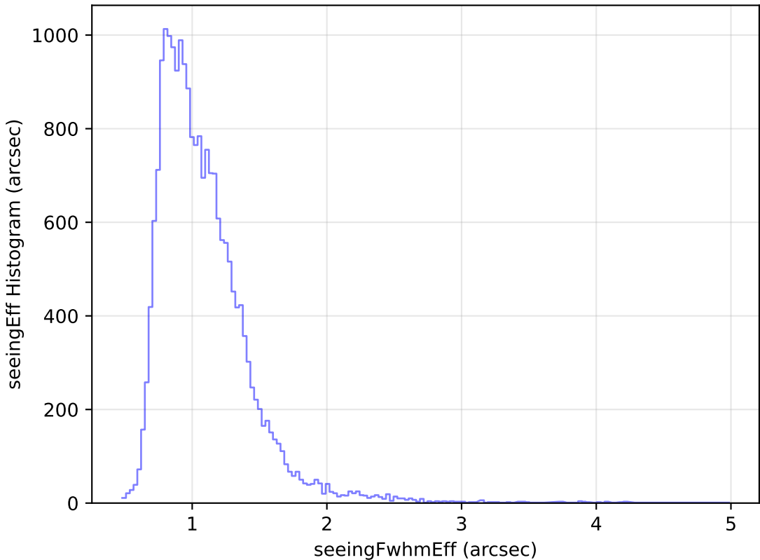
weather_cloudso8v3.4_10yrs Yr 1 g band: seeingEff Histogram
