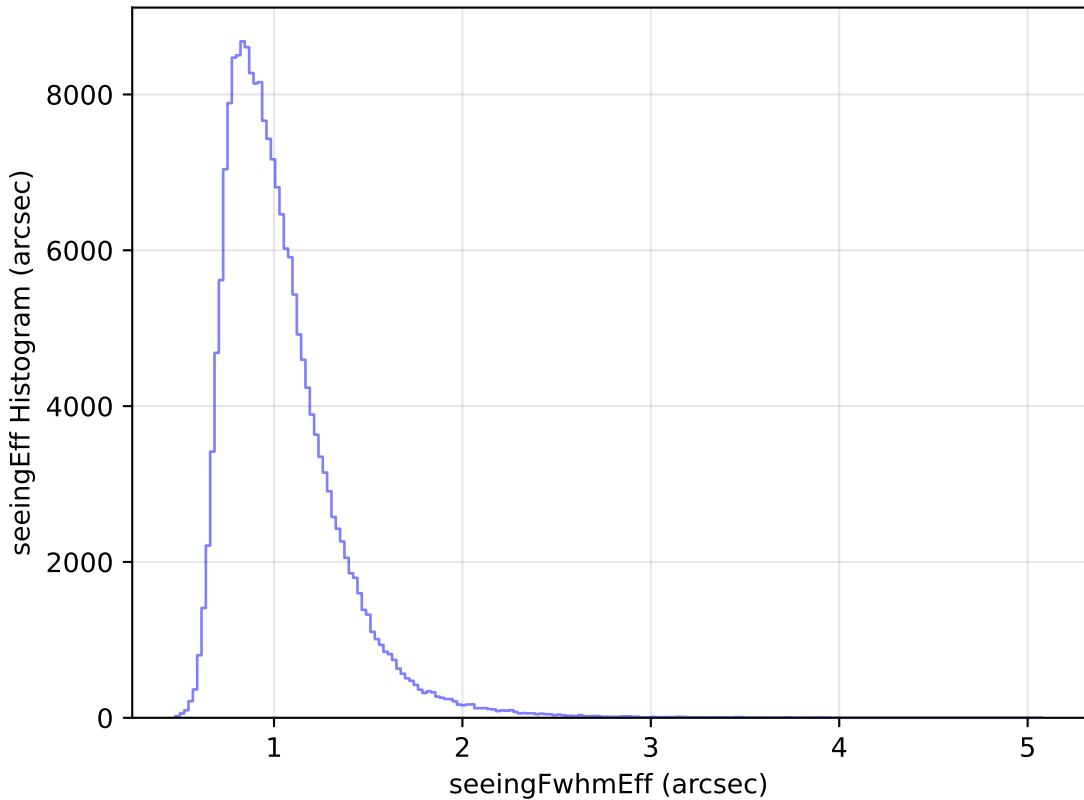
weather_cloudso8v3.4_10yrs Yr 1 all bands: seeingEff Histogram
