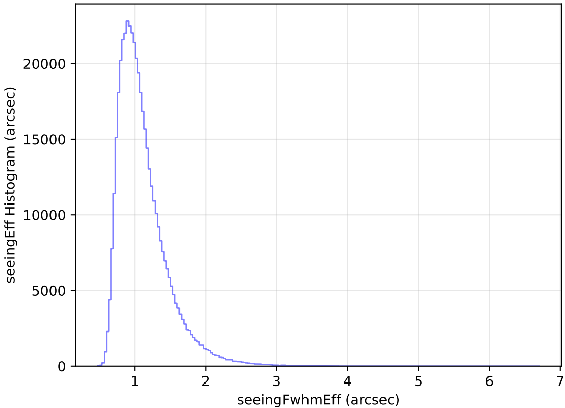
weather_cloudso8v3.4_10yrs WFD z band: seeingEff Histogram
