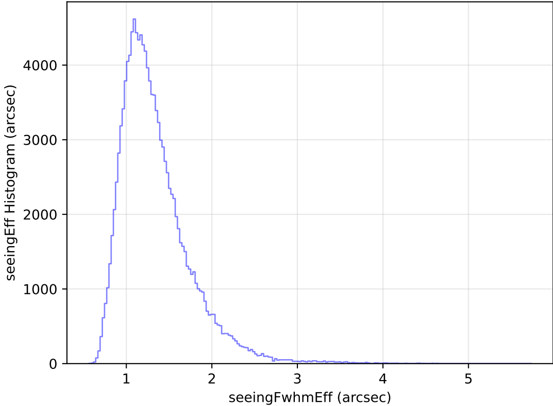
weather_cloudso8v3.4_10yrs WFD u band: seeingEff Histogram
