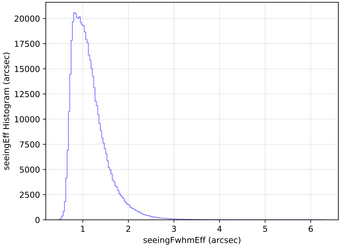
weather_cloudso8v3.4_10yrs WFD r band: seeingEff Histogram
