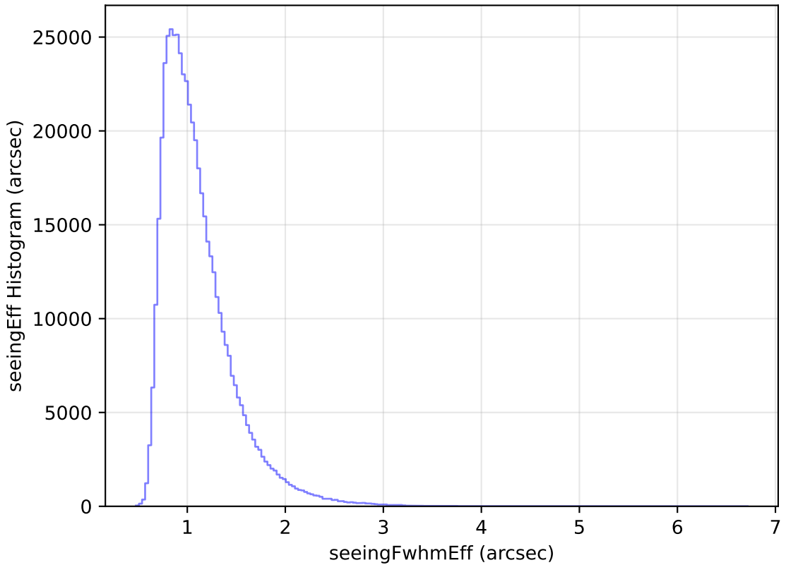
weather_cloudso8v3.4_10yrs WFD i band: seeingEff Histogram
