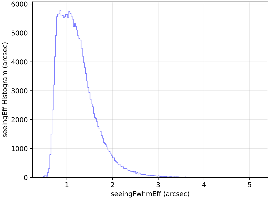
weather_cloudso8v3.4_10yrs WFD g band: seeingEff Histogram
