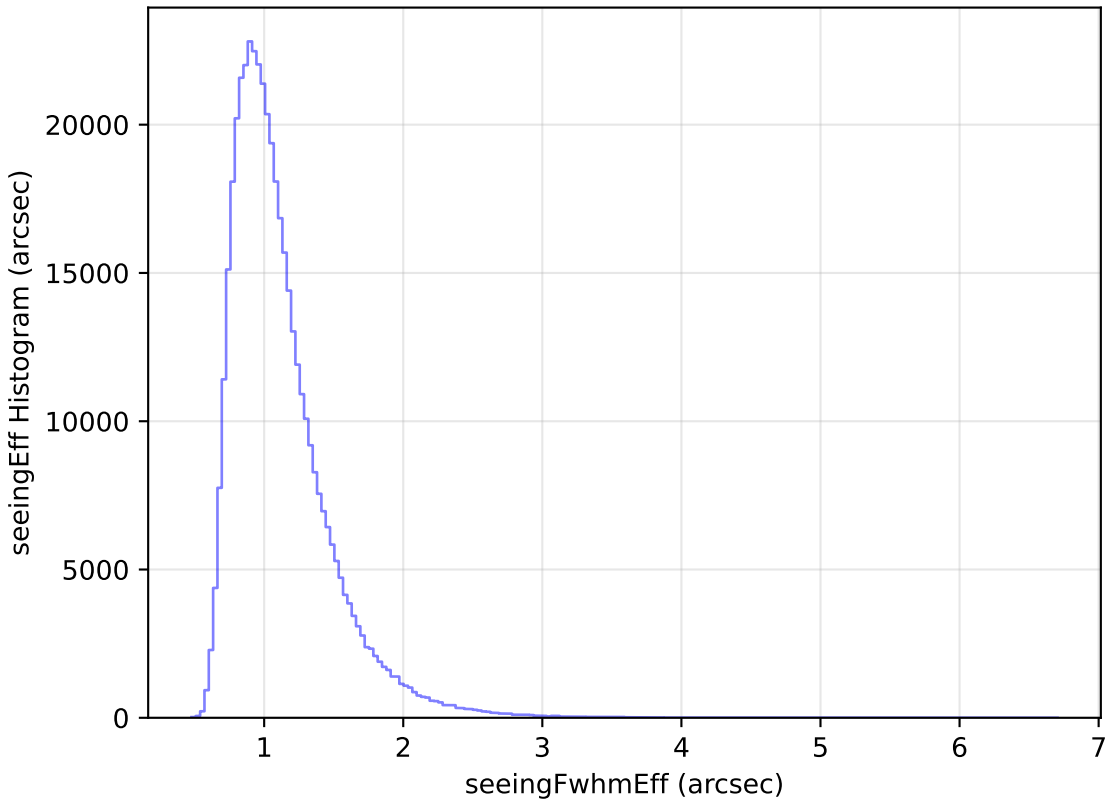
weather_cloudso8v3.4_10yrs All sky z band: seeingEff Histogram
