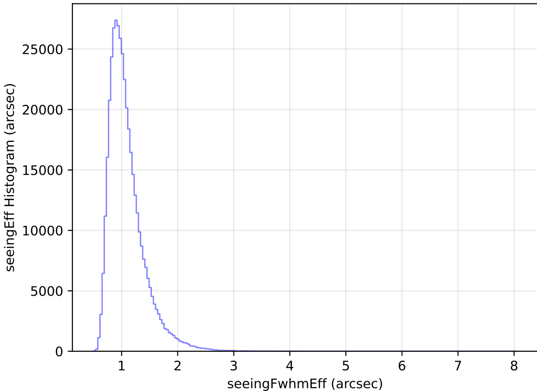
weather_cloudso8v3.4_10yrs All sky y band: seeingEff Histogram
