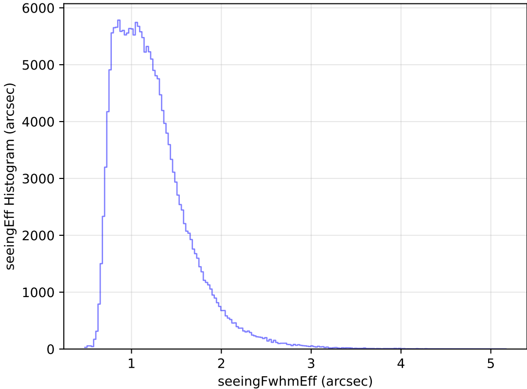
weather_cloudso8v3.4_10yrs All sky g band: seeingEff Histogram
