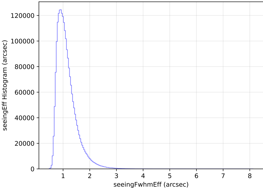
weather_cloudso8v3.4_10yrs All sky all bands: seeingEff Histogram
