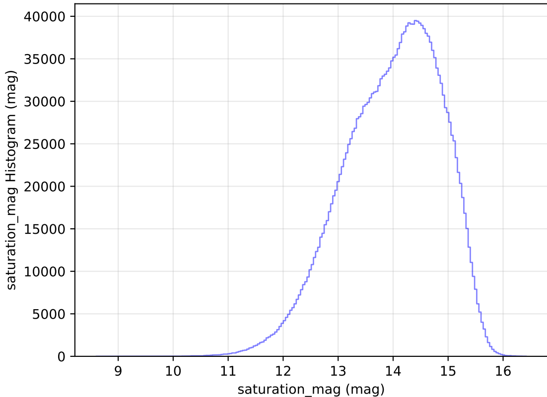
weather_cloudso8v3.4_10yrs WFD all bands: saturation_mag Histogram
