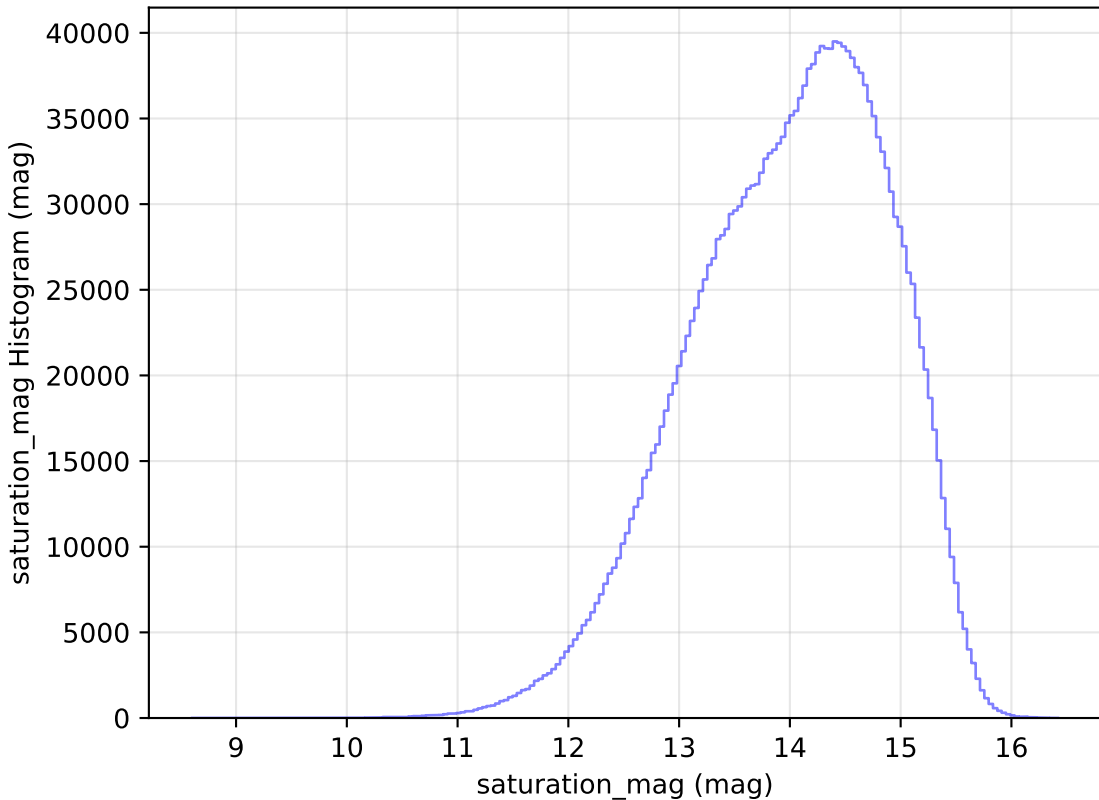
weather_cloudso8v3.4_10yrs All sky all bands: saturation_mag Histogram
