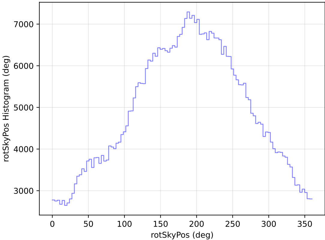
weather_cloudso8v3.4_10yrs WFD r band: rotSkyPos Histogram
