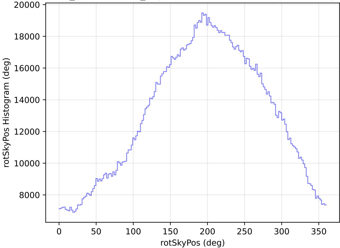
weather_cloudso8v3.4_10yrs WFD all bands: rotSkyPos Histogram
