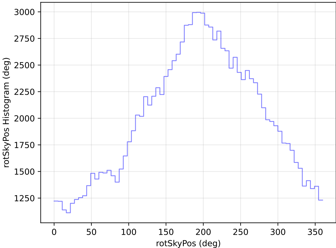
weather_cloudso8v3.4_10yrs All sky u band: rotSkyPos Histogram
