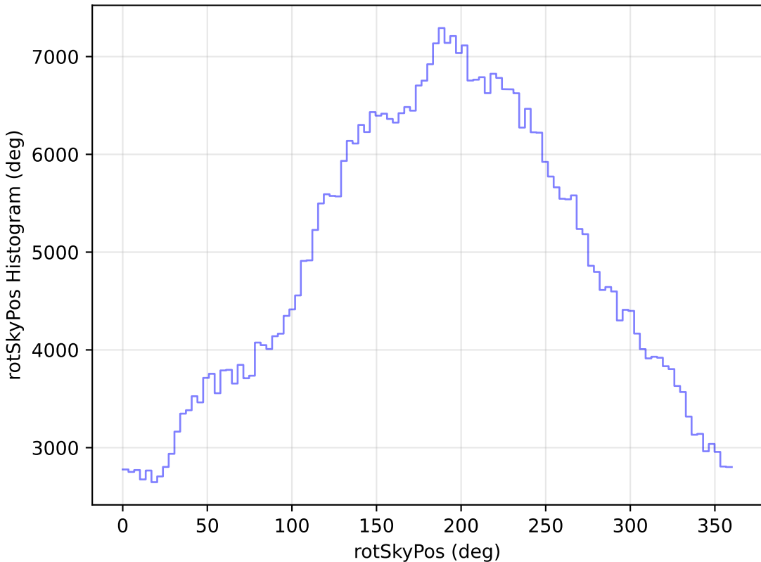
weather_cloudso8v3.4_10yrs All sky r band: rotSkyPos Histogram
