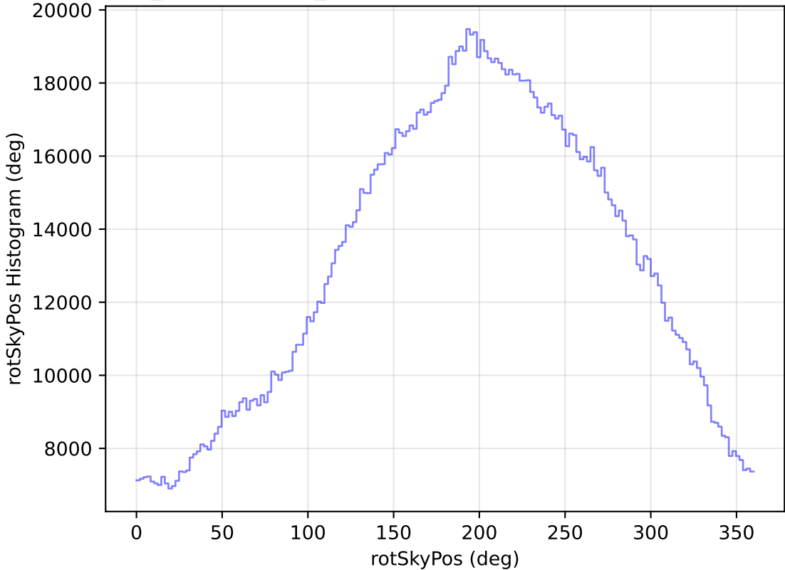
weather_cloudso8v3.4_10yrs All sky all bands: rotSkyPos Histogram
