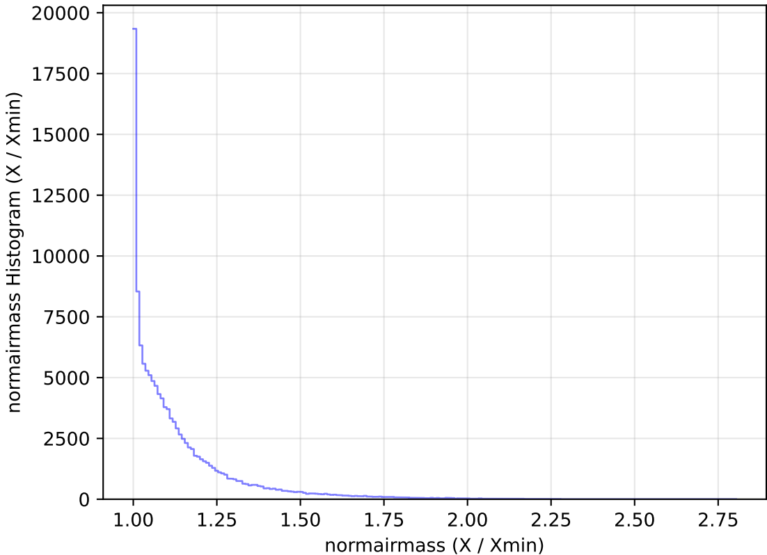
weather_cloudso8v3.4_10yrs WFD u band: normairmass Histogram
