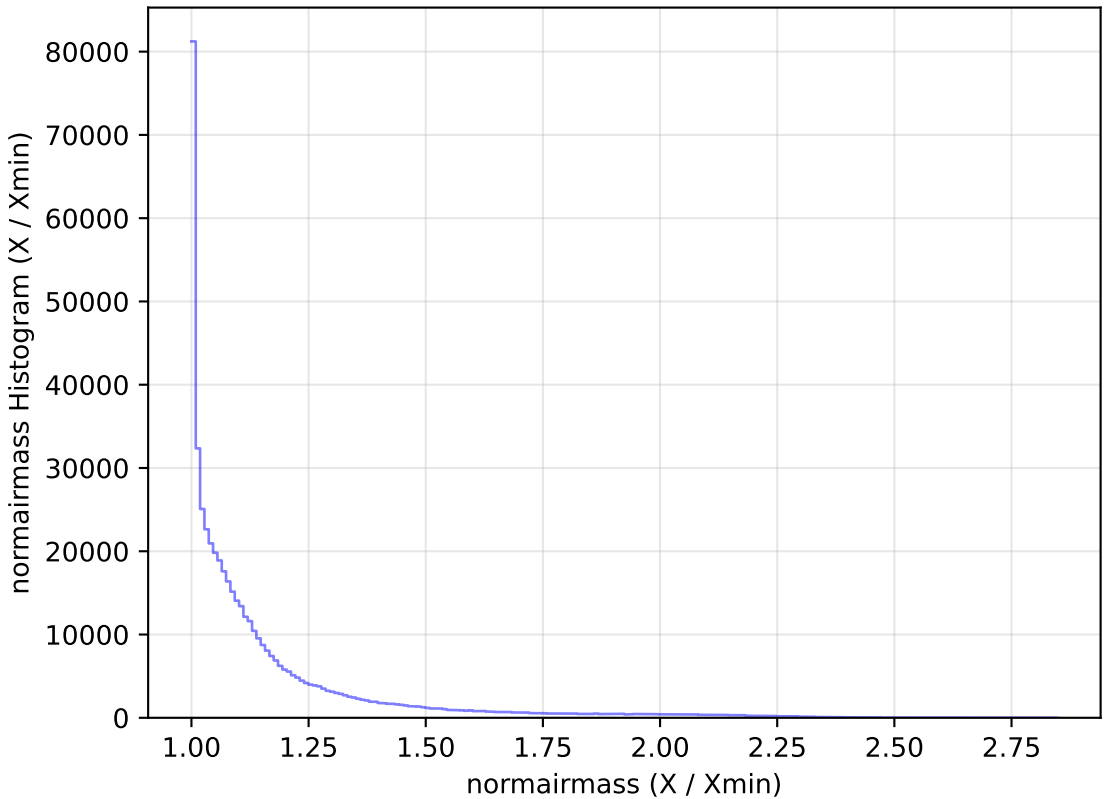
weather_cloudso8v3.4_10yrs WFD r band: normairmass Histogram
