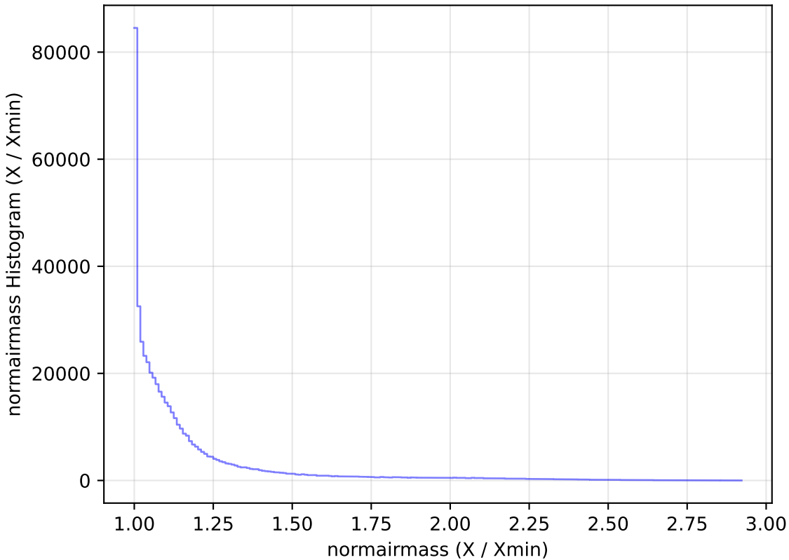
weather_cloudso8v3.4_10yrs WFD i band: normairmass Histogram
