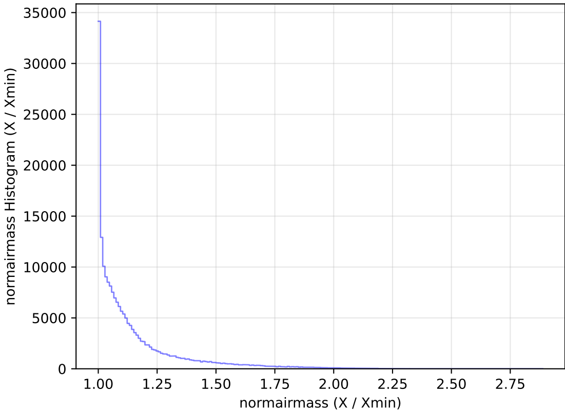
weather_cloudso8v3.4_10yrs WFD g band: normairmass Histogram
