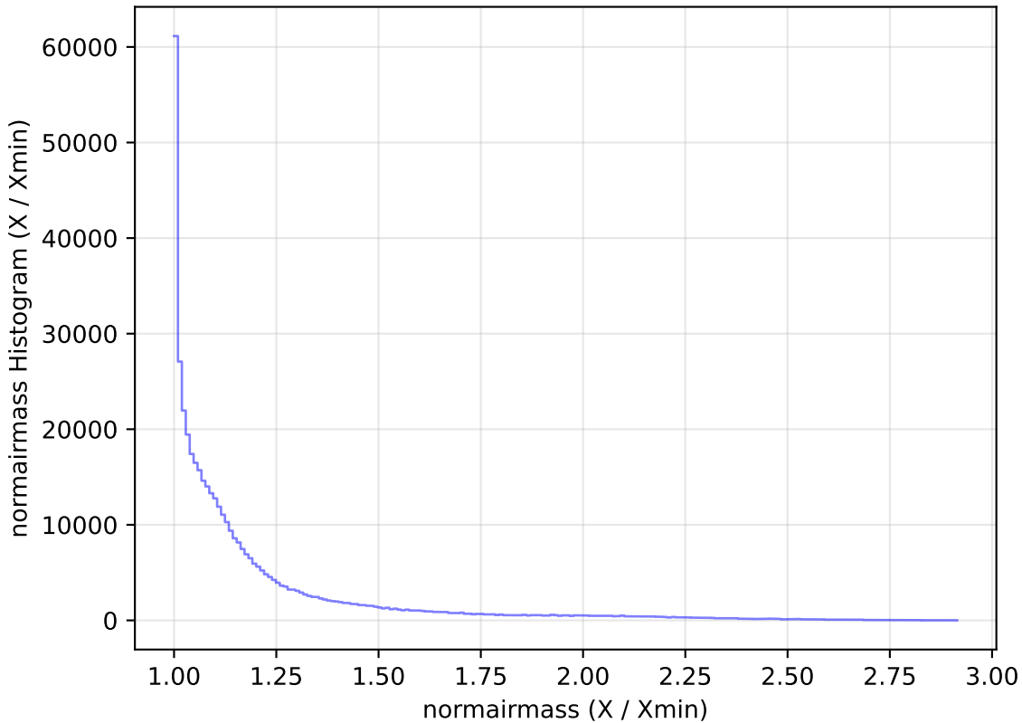
weather_cloudso8v3.4_10yrs All sky z band: normairmass Histogram
