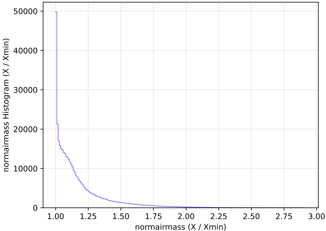
weather_cloudso8v3.4_10yrs All sky y band: normairmass Histogram
