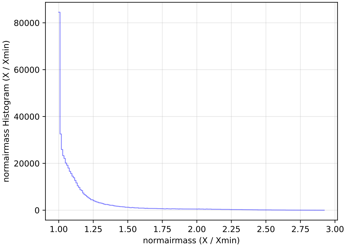
weather_cloudso8v3.4_10yrs All sky i band: normairmass Histogram
