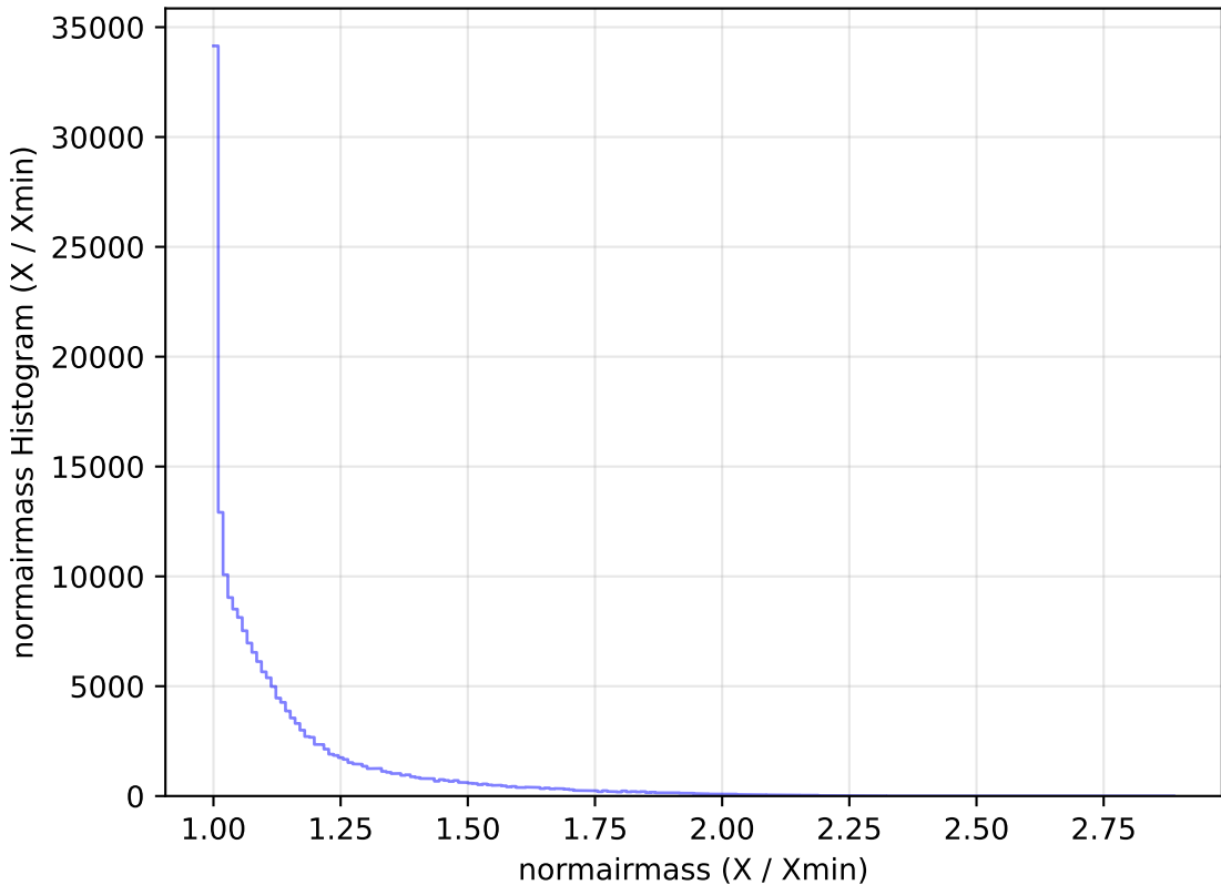
weather_cloudso8v3.4_10yrs All sky g band: normairmass Histogram
