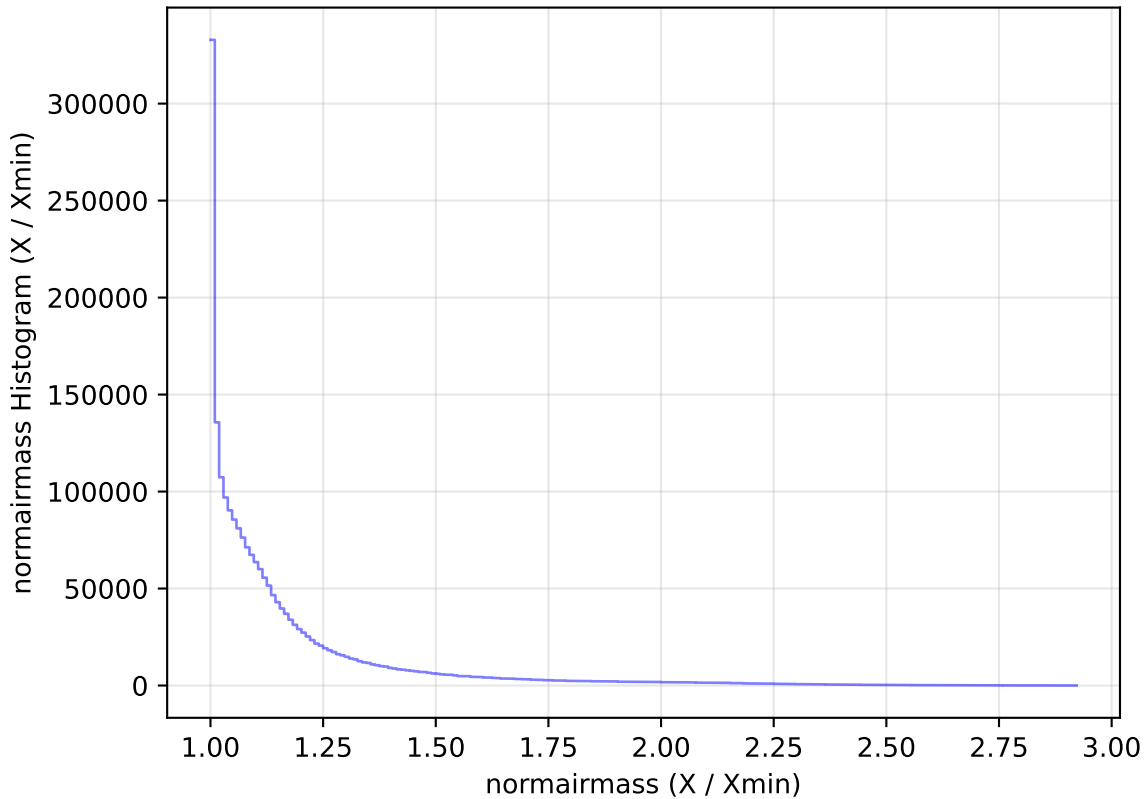
weather_cloudso8v3.4_10yrs All sky all bands: normairmass Histogram
