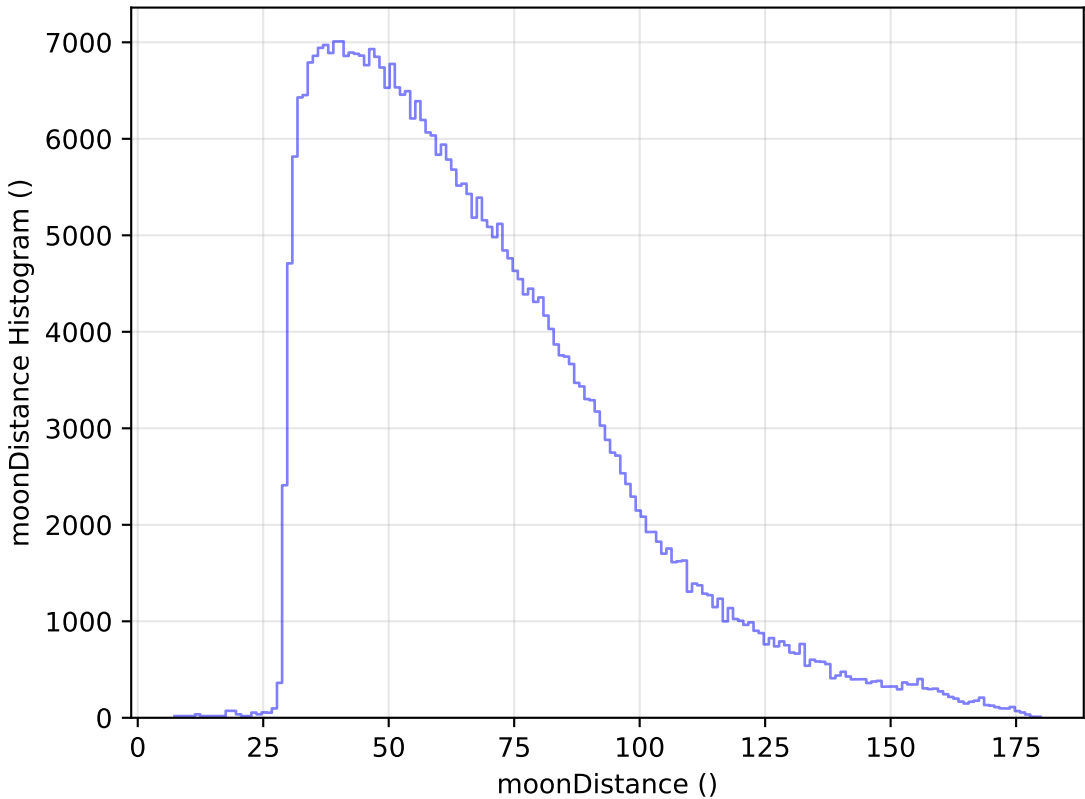
weather_cloudso8v3.4_10yrs WFD y band: moonDistance Histogram
