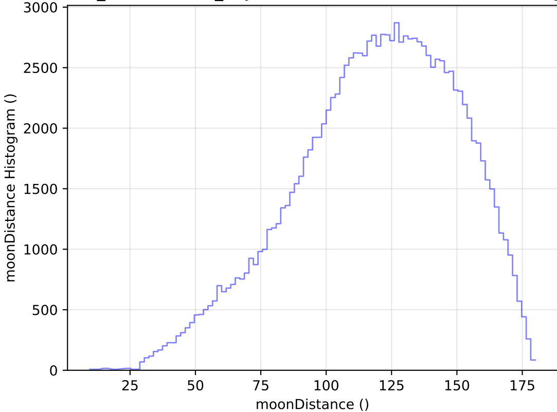
weather_cloudso8v3.4_10yrs WFD u band: moonDistance Histogram
