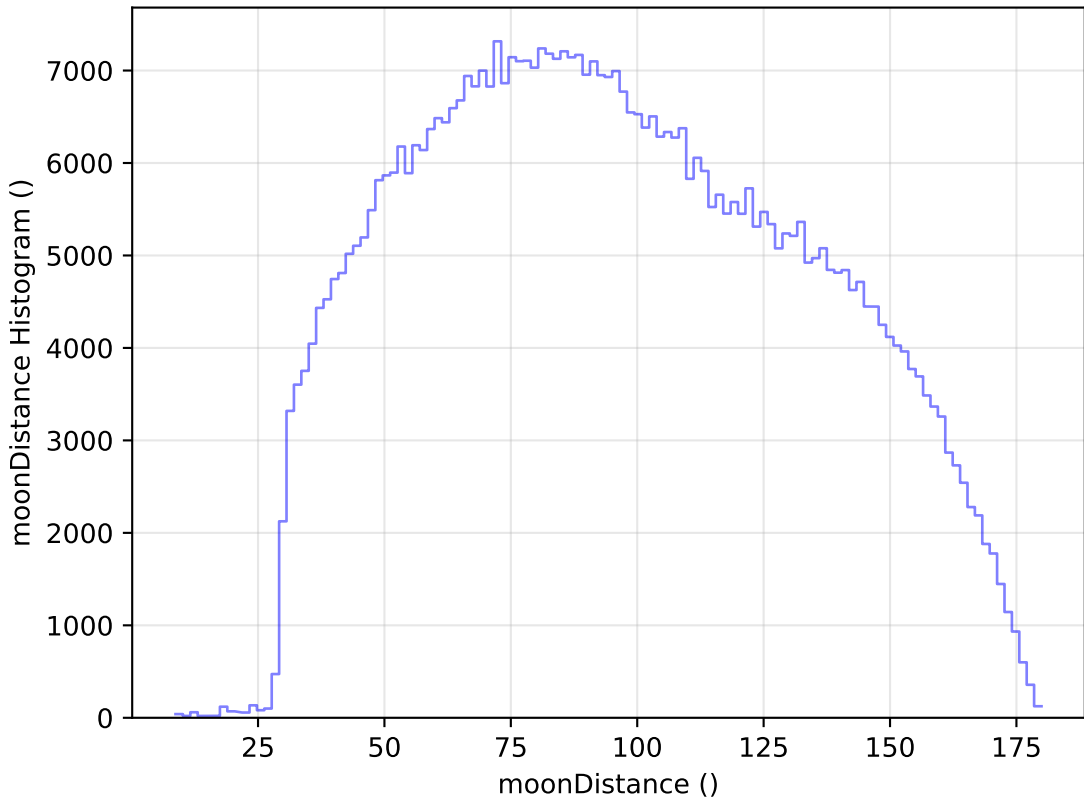
weather_cloudso8v3.4_10yrs WFD i band: moonDistance Histogram
