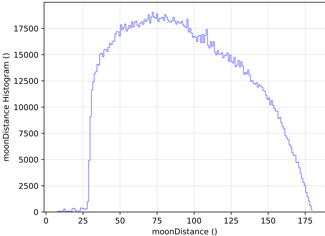
weather_cloudso8v3.4_10yrs WFD all bands: moonDistance Histogram
