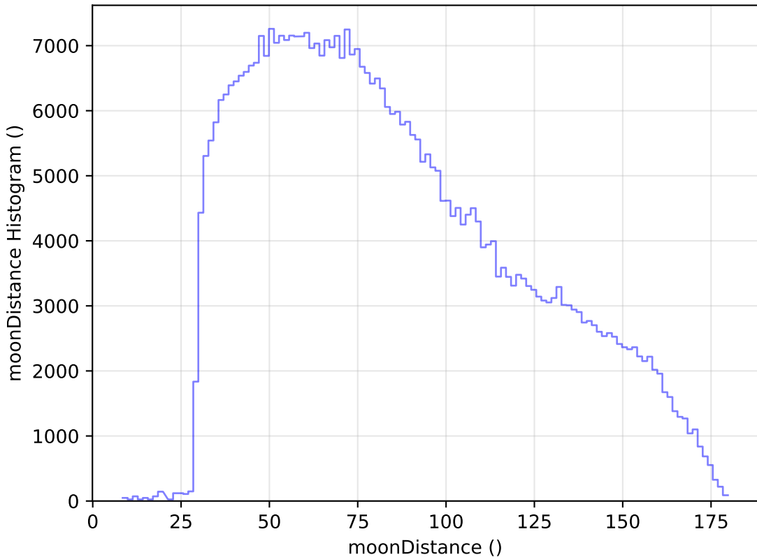
weather_cloudso8v3.4_10yrs All sky z band: moonDistance Histogram
