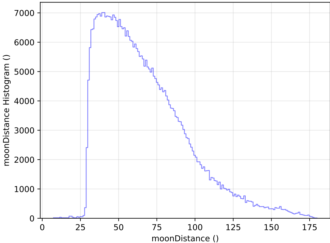
weather_cloudso8v3.4_10yrs All sky y band: moonDistance Histogram
