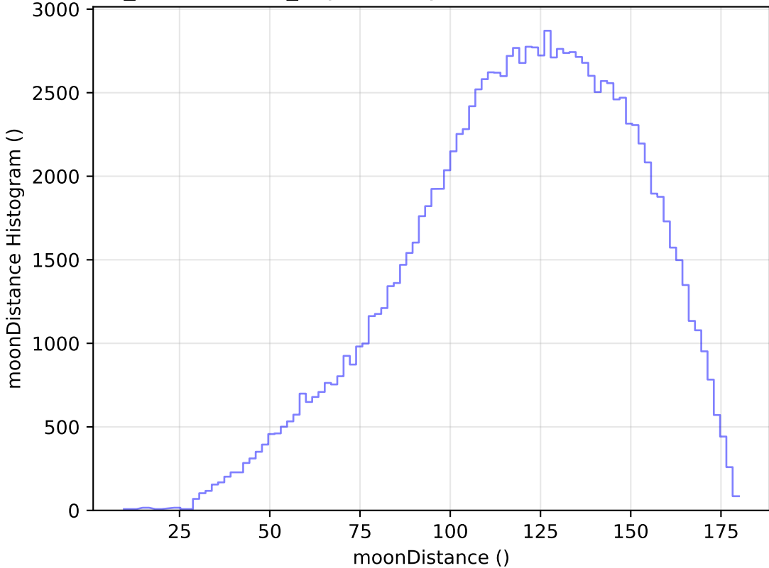
weather_cloudso8v3.4_10yrs All sky u band: moonDistance Histogram
