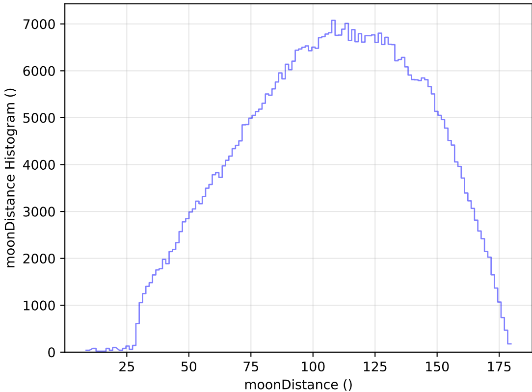
weather_cloudso8v3.4_10yrs All sky r band: moonDistance Histogram
