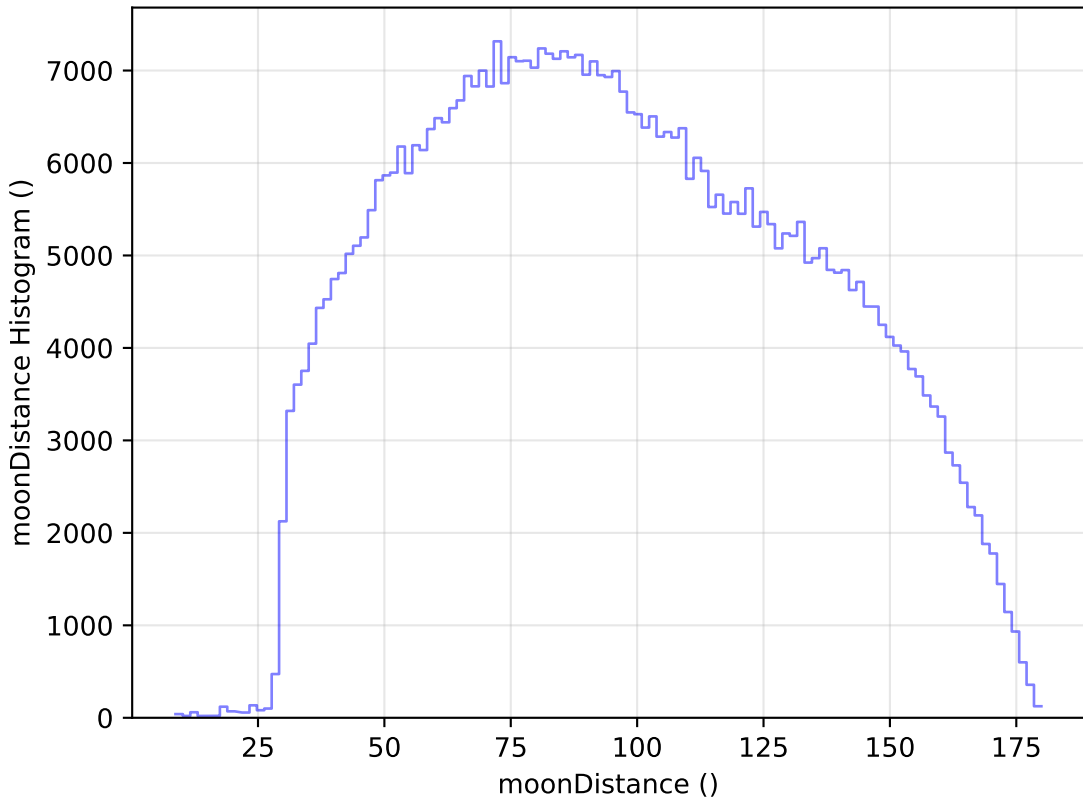
weather_cloudso8v3.4_10yrs All sky i band: moonDistance Histogram
