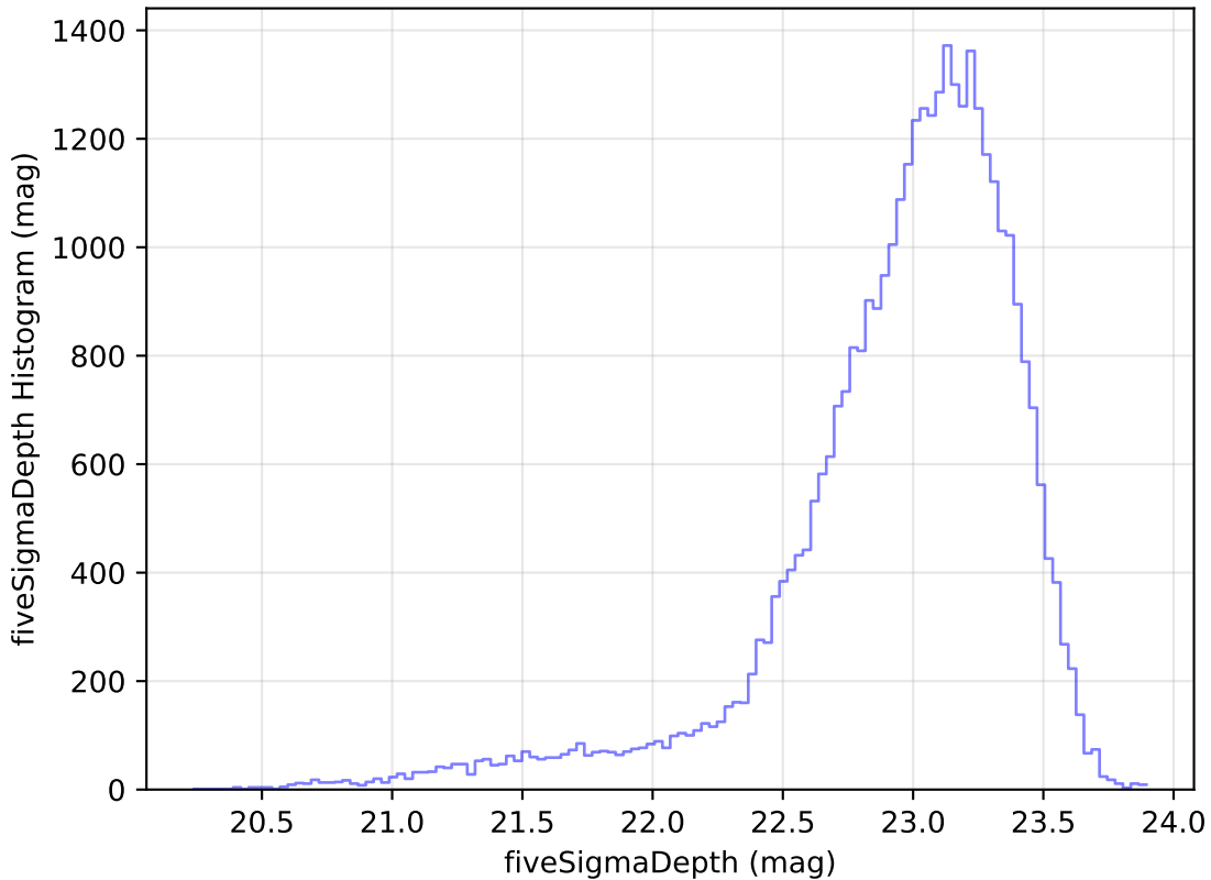
weather_cloudso8v3.4_10yrs Yr 1 z band: fiveSigmaDepth Histogram
